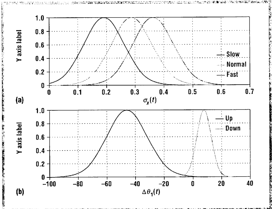
Figure 6. Membership functions of (a) input \sigma_x(t) for level behaviors and (b) input \Delta\theta_1(t) for up and down behaviors.
