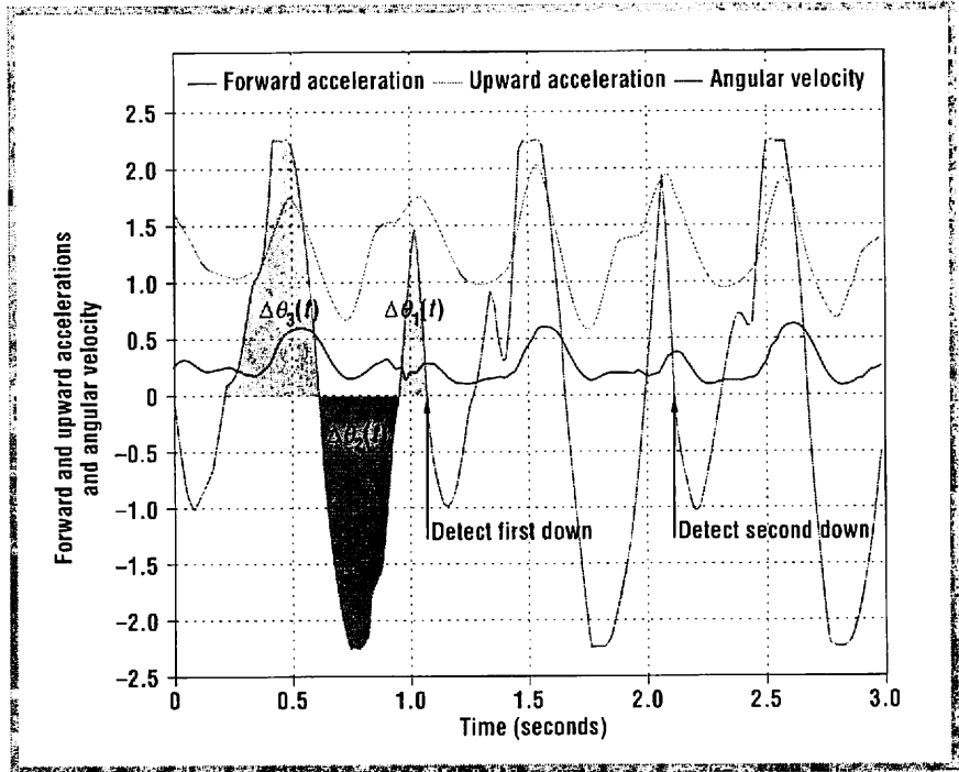
Figure 3. Typical trajectories of sensor signals for level walking behavior of two subjects.
