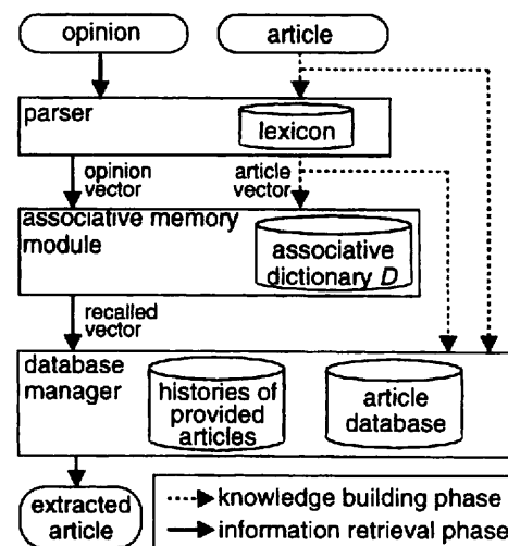
Fig. 4. Software structure and process flow of the prototype system.
